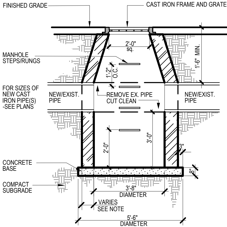
SECTION B-B
