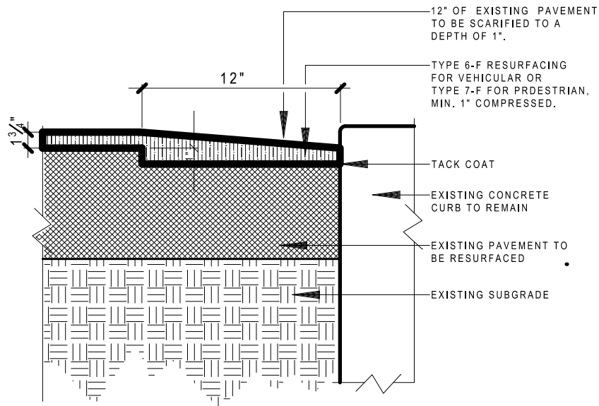
ASPHALT RESURFACING at Concrete Curb
