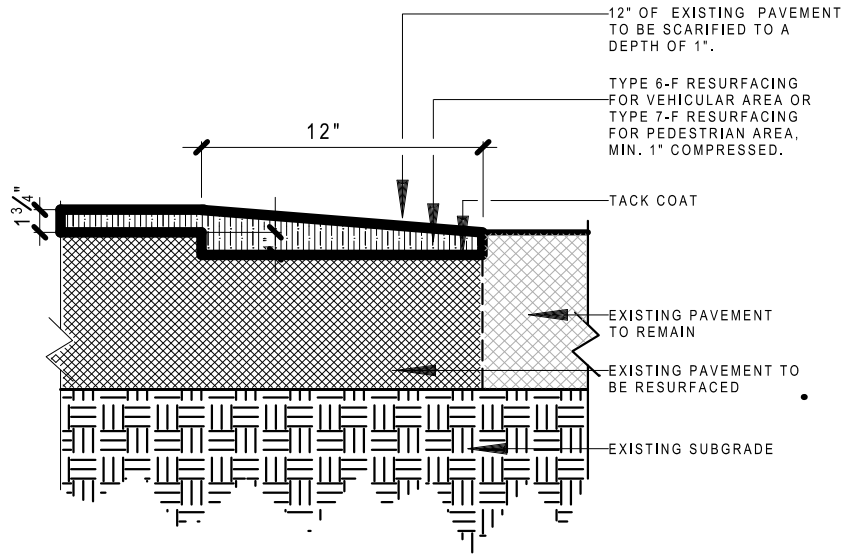
ASPHALT RESURFACING at Existing Pavement
