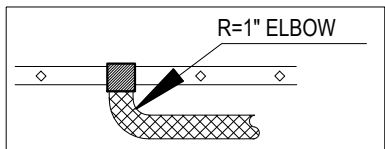
PLAN OF HANDRAIL TO POST CONNECTION
