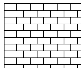
RUNNING BOND PATTERN
