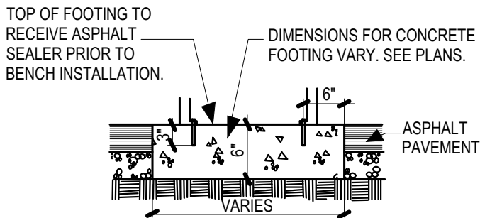
SECTION VIEW
