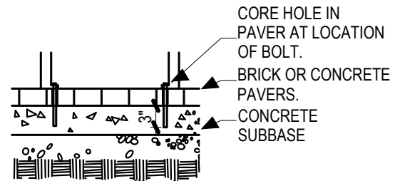
SECTION VIEW
