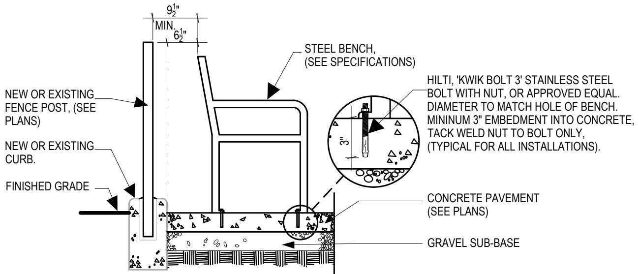
SECTION VIEW
