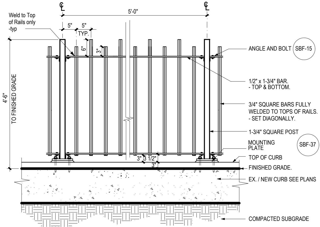
ELEVATION / SECTION
