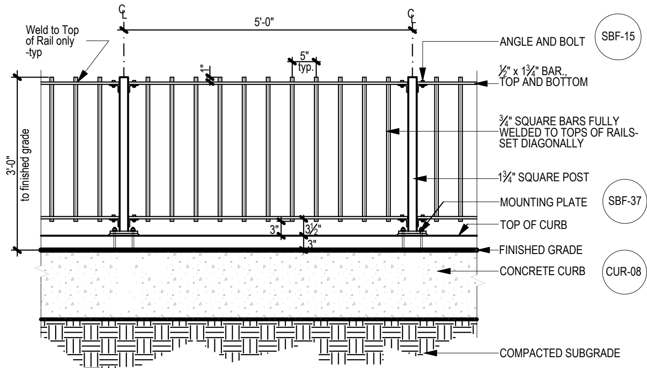
ELEVATION / SECTION
