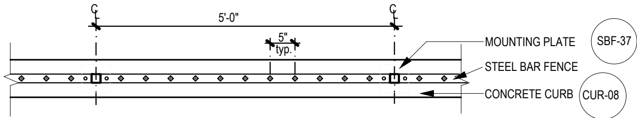
PLAN
