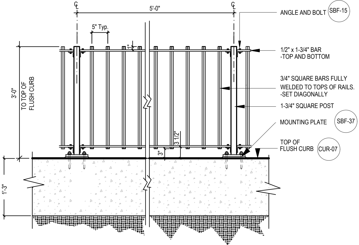
SECTION/ELEVATION
