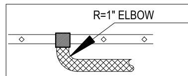
PLAN OF HANDRAIL TO POST CONNECTION
