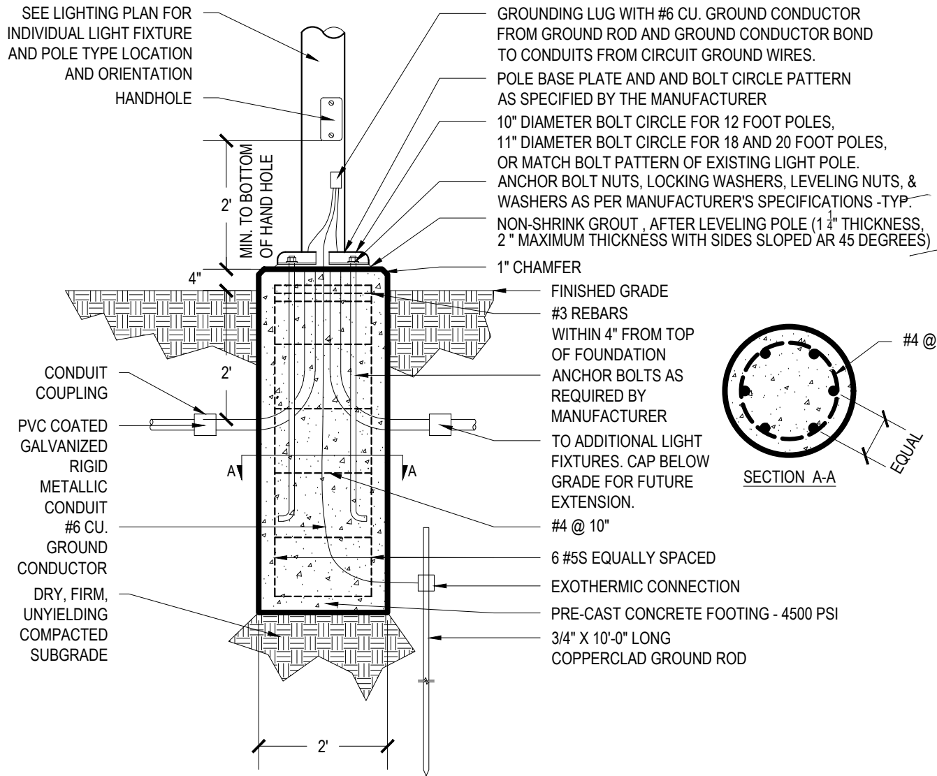
Light Pole Foundation, Pole Base & Grounding Detail at Planted Areas
