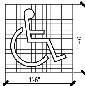
SYMBOL PROPORTIONS
