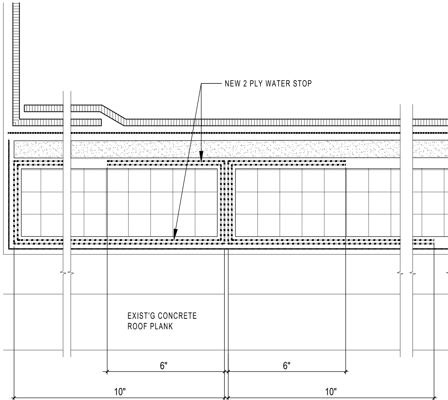
WATER STOP DETAIL @ VERTICAL PROJECTIONS
