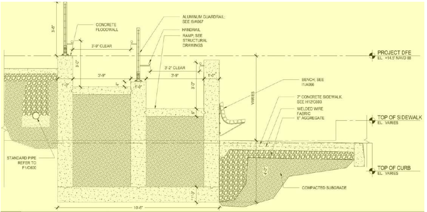
A1 TYPICAL FLOODWALL RAMP SECTION
