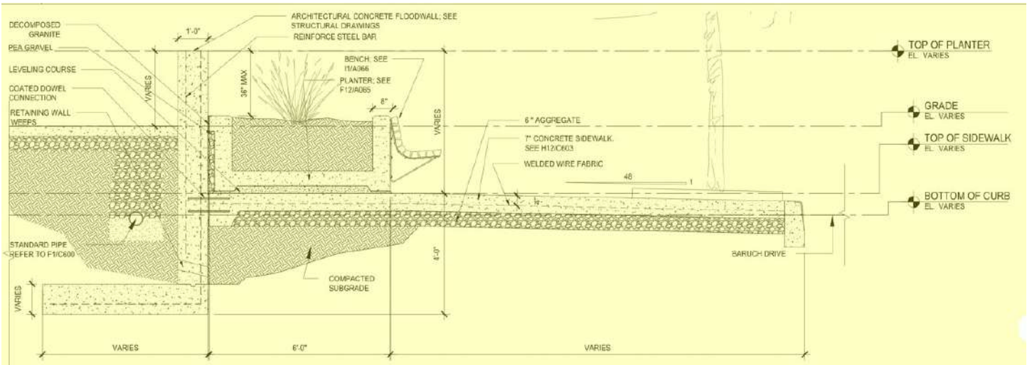
E1 TYPICAL FLOODWALL PLANTER SECTION
