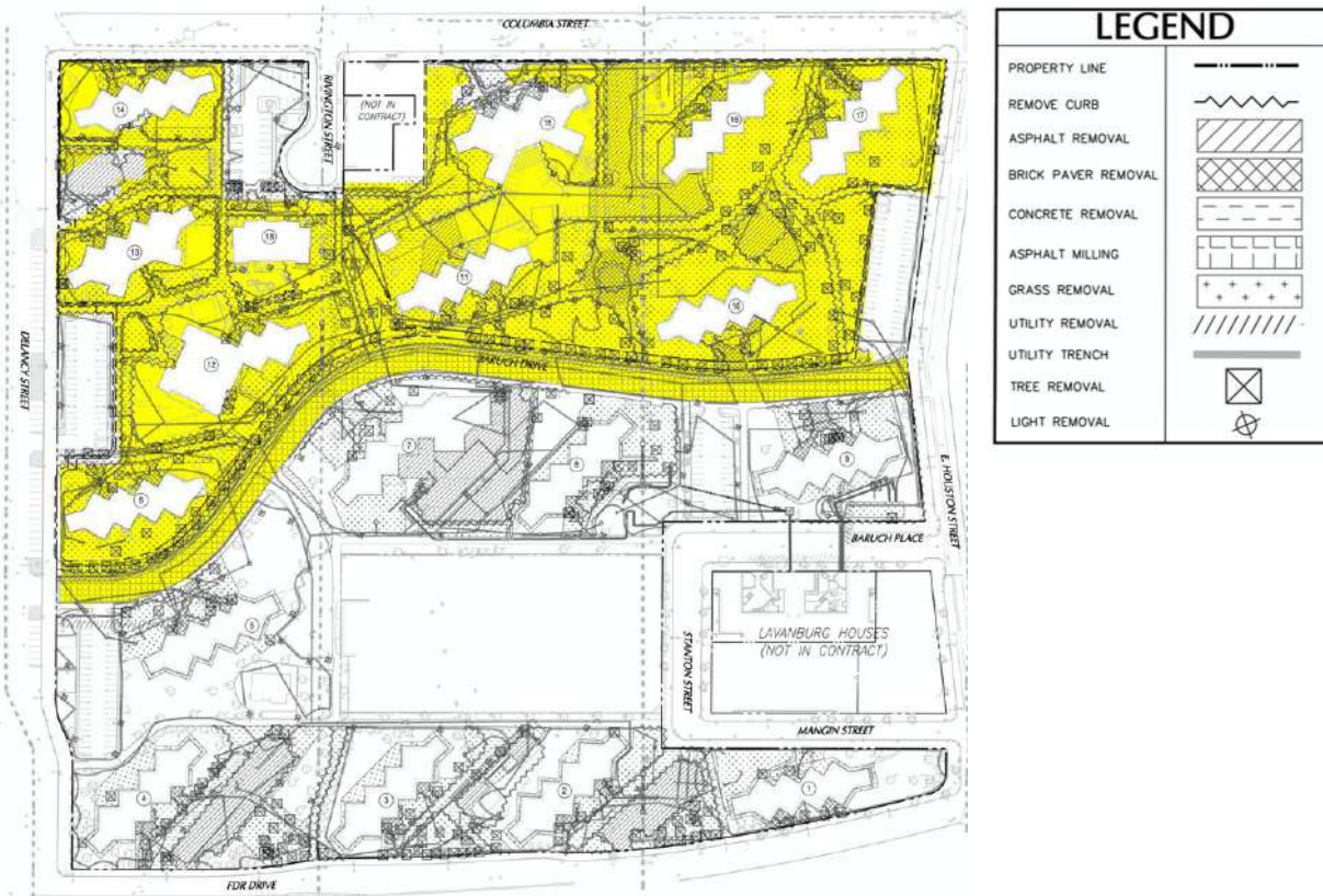
Baruch site removal plan
